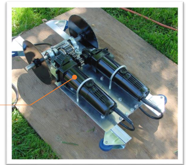
Power tool dragster designed and built for the first and only Sacramento power tool dragster competition. Two angle grinders, spur gear powertrain, and saw blade rear wheels
